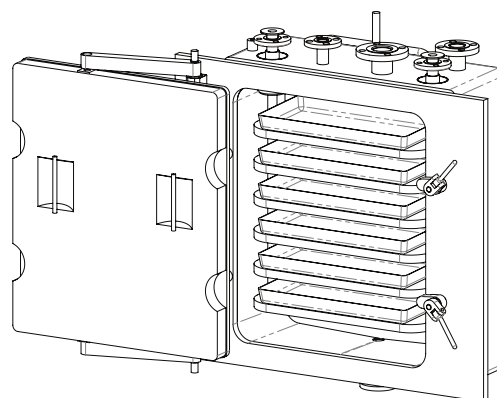
Example of a module for CakeStand within PSL glovebox
