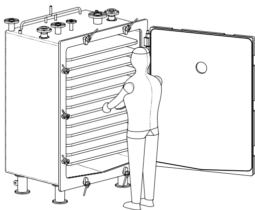
Example of a free-standing CakeStand tray dryer
