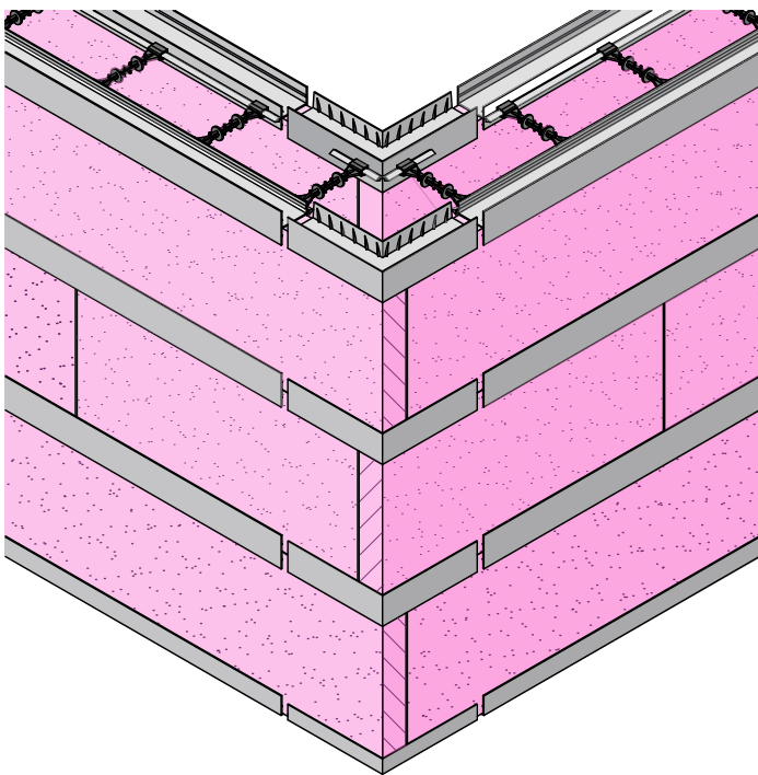
WALL CORNER SHOWING FOAM SLABS LAID IN ALTERNATE DIRECTIONS
