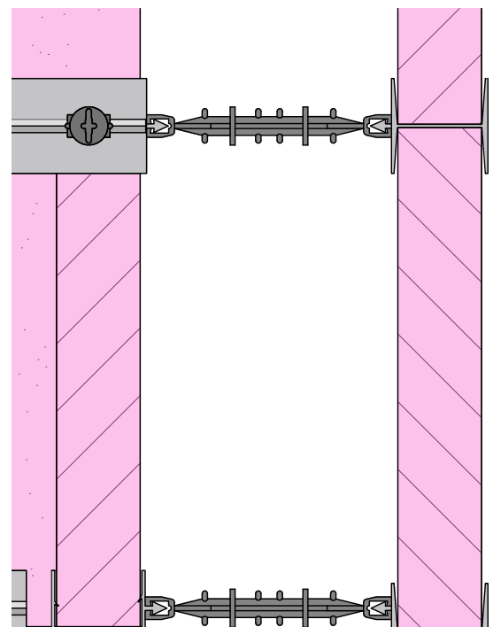
SECTION THROUGH CAVITY SHOWING TIES, RAILS AND FOAM BLOCKS SHOWING 50MM BOARDS
