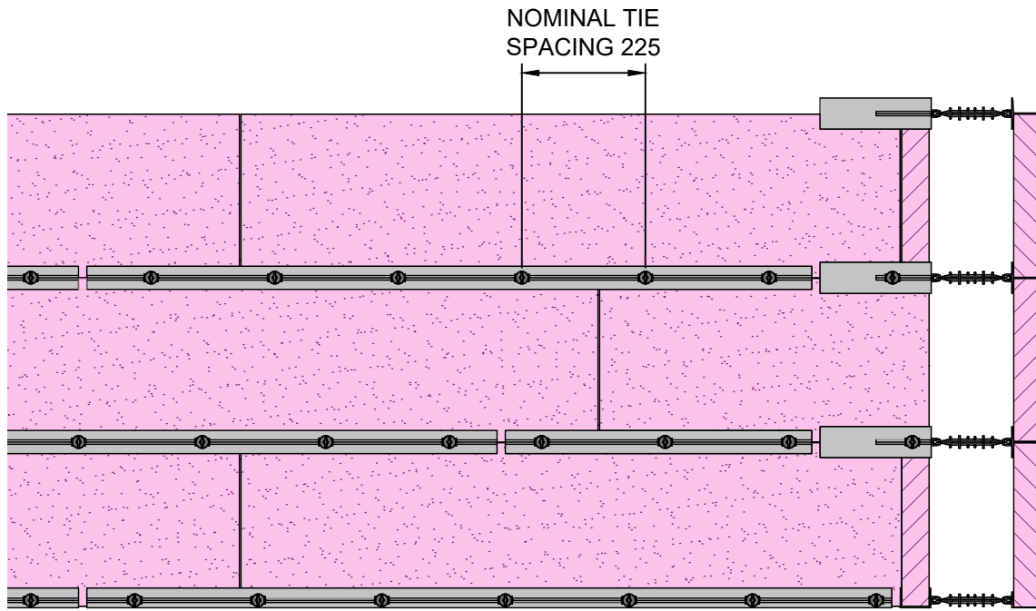
SECTION THROUGH CAVITY AT WALL CORNER
