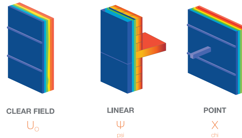
Examples of thermal transmittance and heat flow through the building envelope. Steel girts can be seen in the clear field wall assembly, a steel shelf angle bolted to a slab edge as an example of a linear detail and a single beam penetrating the envelope as a point detail. (Source: Morrison Hershfield)
