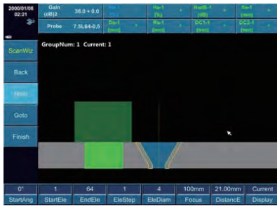
Beam Coverage Simulation(Single Probe)
