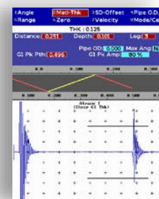
Shear mode (flat + curved)
