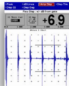
TCG - Time Corrected Gain
