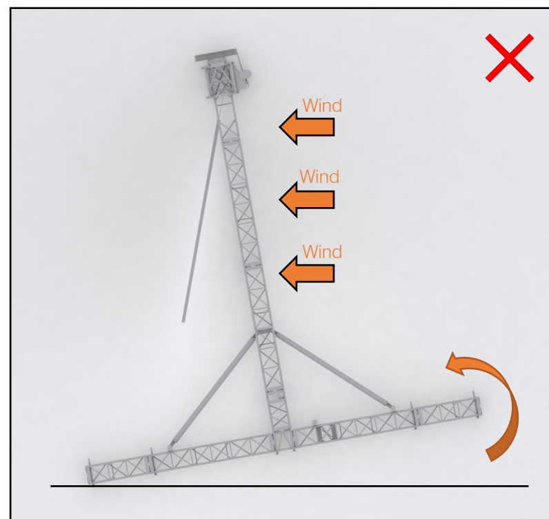
Fig. 34 - Wind Load Stability (18.1)
