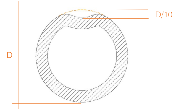
Fig. 37 – Dents (20.3.6)
