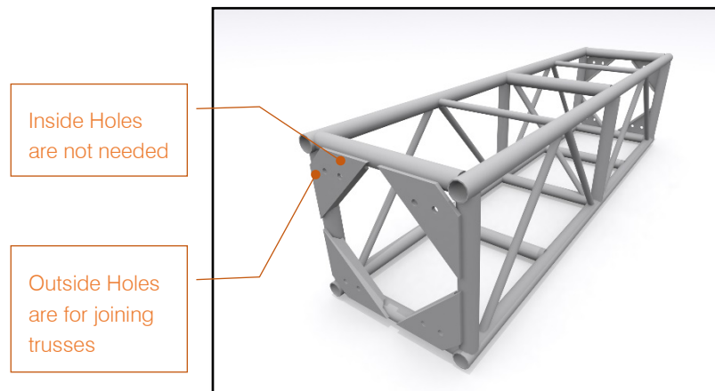
Fig. 47 - Medium Duty Truss (24.5.1)
