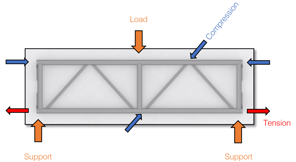
Fig. 1 – Forces (7.2)
