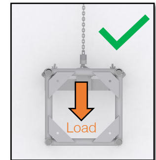
Fig. 22 - Load evenly (12.3.8)
