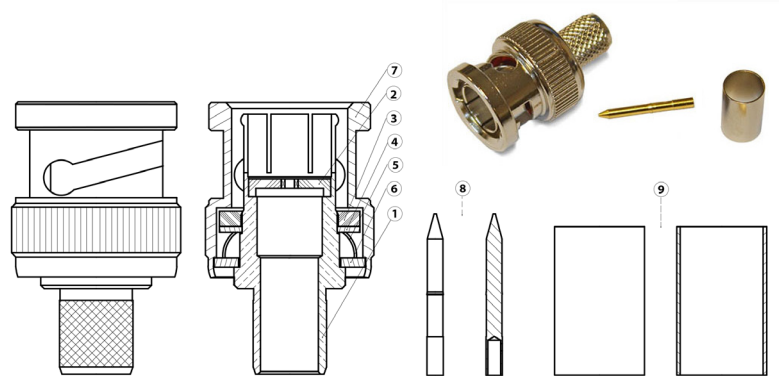
1 - Body 2 - Insulator 3 - Gasket 4 - Spring 5 - C Ring 6 - Washer 7 - Shell 8 - Contact Pin 9 - Ferrule
