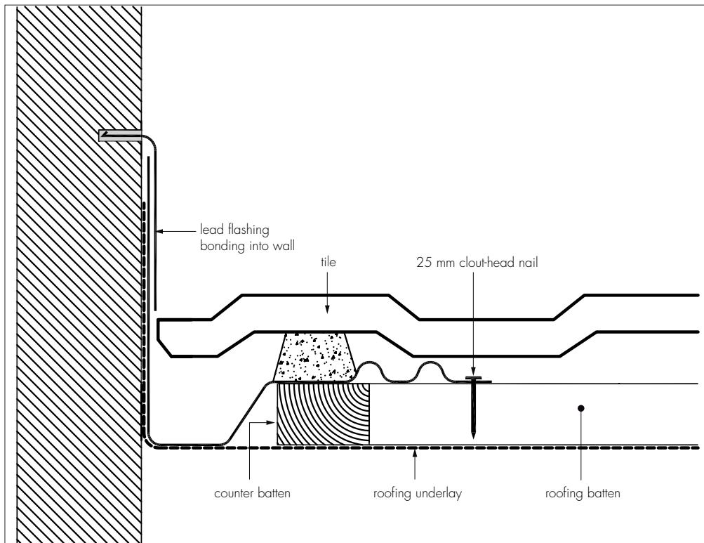
Figure 1 Filon GRP Abutment Secret Gutter/Soaker (GAS 1)
