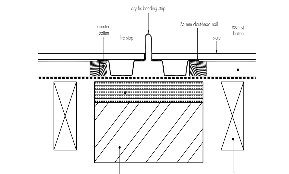
Figure 1 Filon GRP Dry Fix Bonding Strip (GDFBS 70 and GDFBS 110): GDFBS 70
