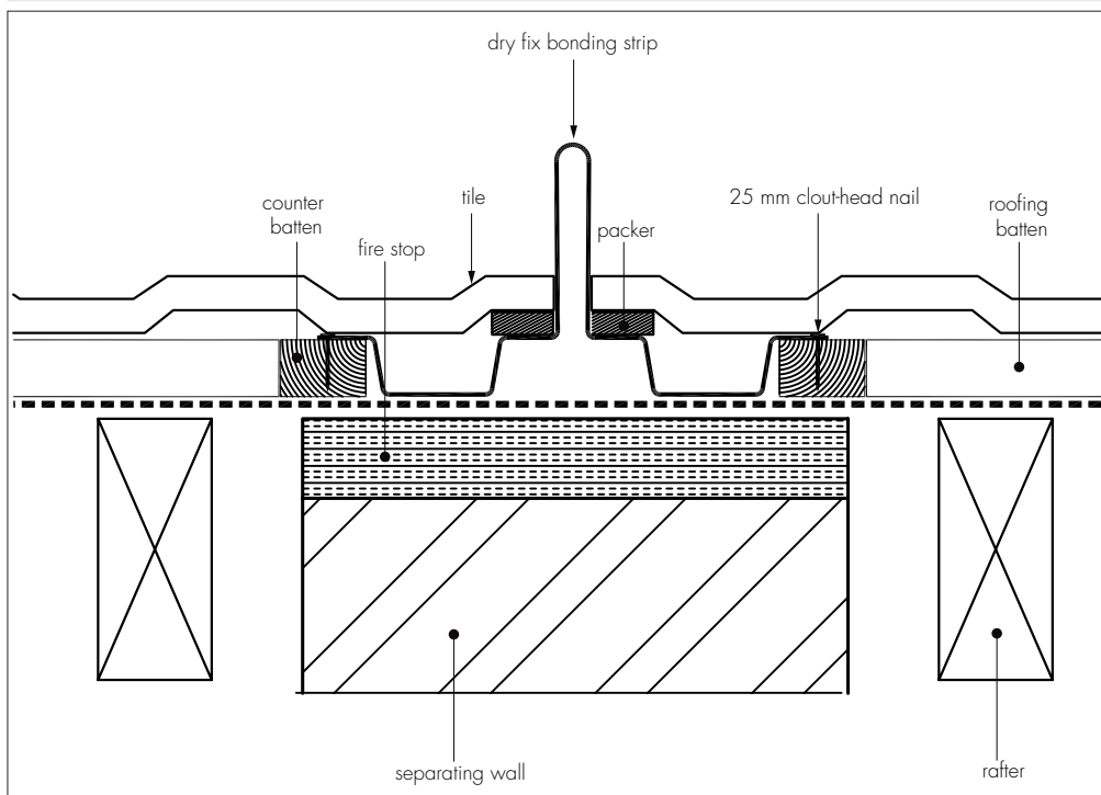
Figure 2 Filon GRP Dry Fix Bonding Strip (GDFBS 70 and GDFBS 110): GDFBS 110
