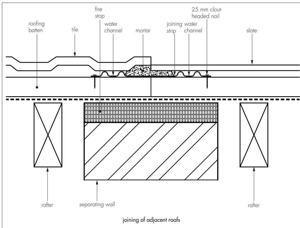
Figure 1 Filon GRP Secret Joining Strip (GJS 1)
