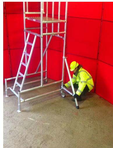
6) FIT STABILISERS TO BACK VERTICALS
