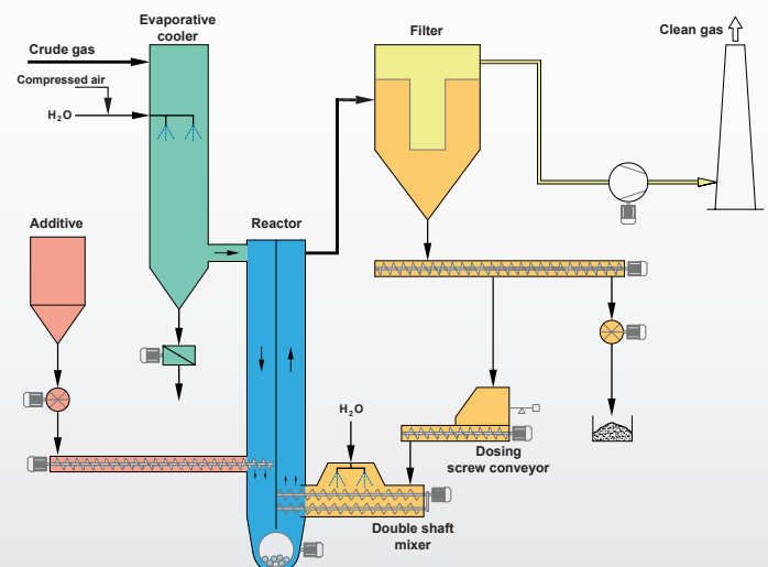
Variants of the Conditioning Rotor-Recycle Process
