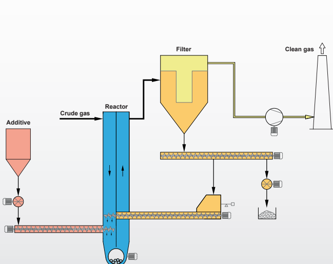
Variants of the Conditioning Rotor-Recycle Process
