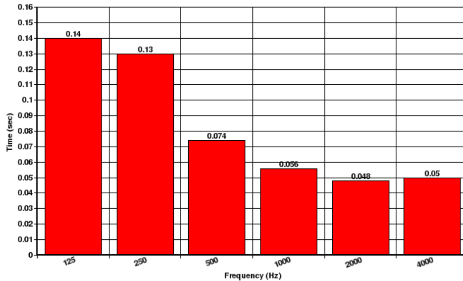
Reverberation Time Inside Silent Space Isolation Booth
