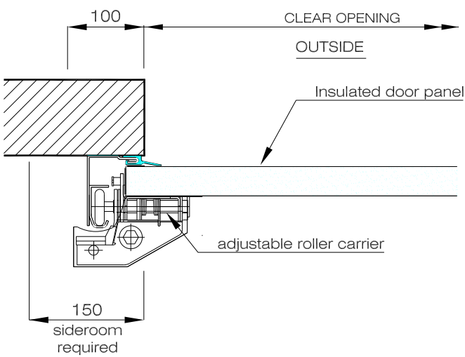
TYPICAL GUIDE FIXING TO STEEL JAMB
