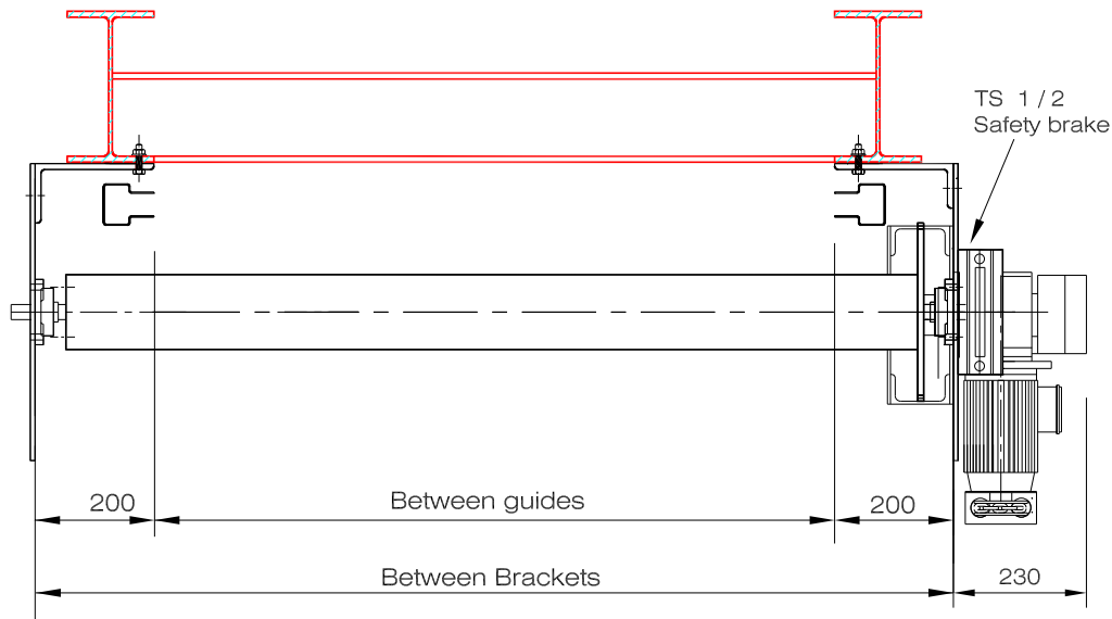
PLAN AT HEAD
