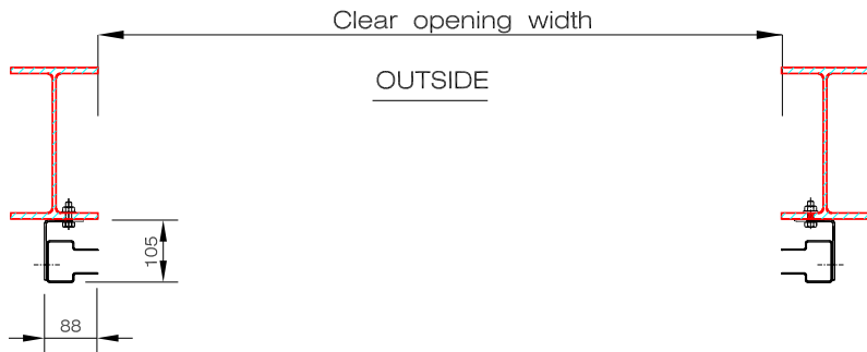
PLAN ON GUIDES
