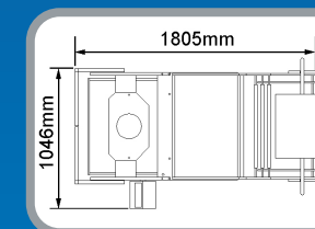
CYCLONE 300
