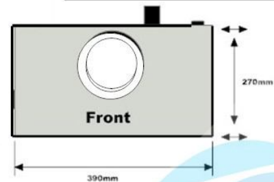
Uniflo Flush 1 Macerator Pump Dimensions
