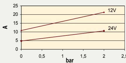
Assorbimenti / Consumption
