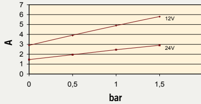
Assorbimenti / Consumption
