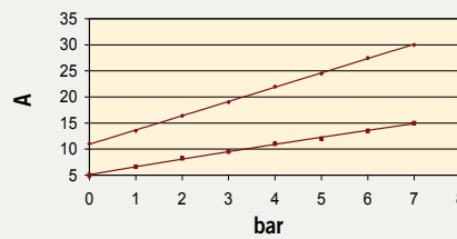
Assorbimenti / Consumption
