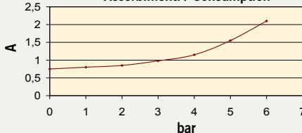
Assorbimenti / Consumption
