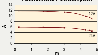
Assorbimenti / Consumption
