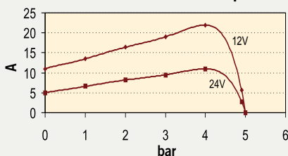
Assorbimenti / Consumption
