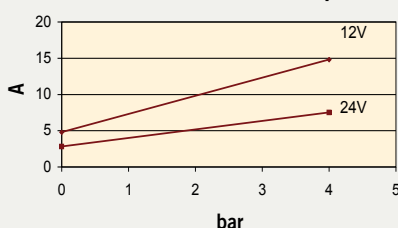
Assorbimenti / Consumption
