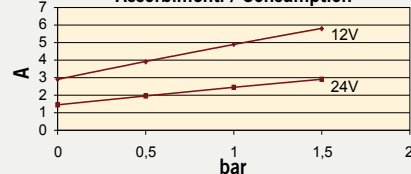
Assorbimenti / Consumption
