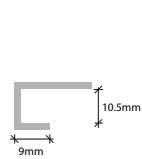
Type U End Cap
