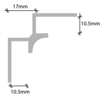
Type V Internal Corner
