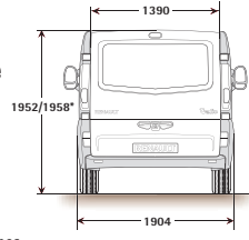
Long wheelbase low roof
