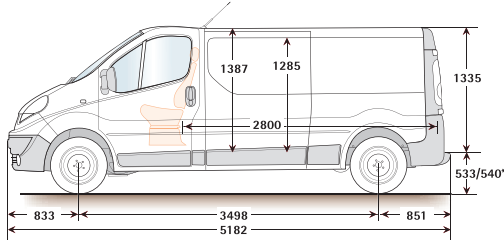
Long wheelbase low roof
