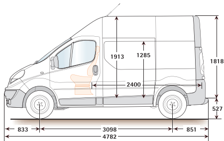
Short wheelbase high roof
