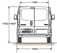
Long wheelbase low roof
