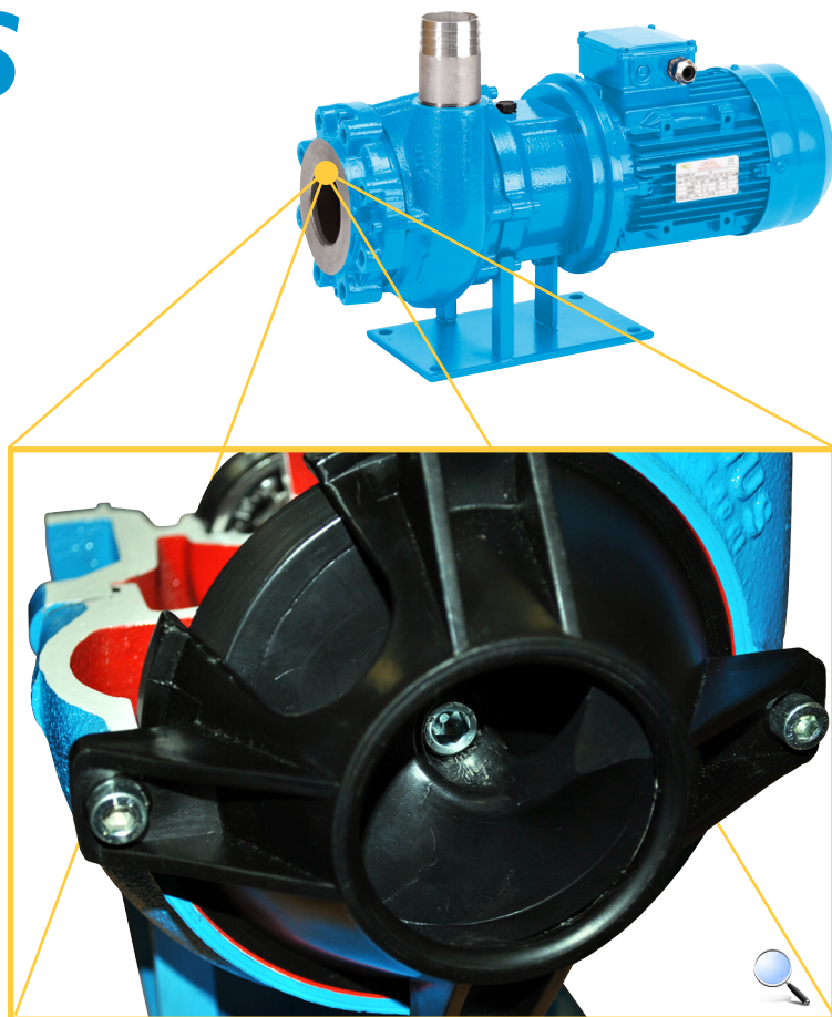
Above: A close-up of a sectioned Verderhus with large open impeller for handling fluids with a high percentage of solids.
