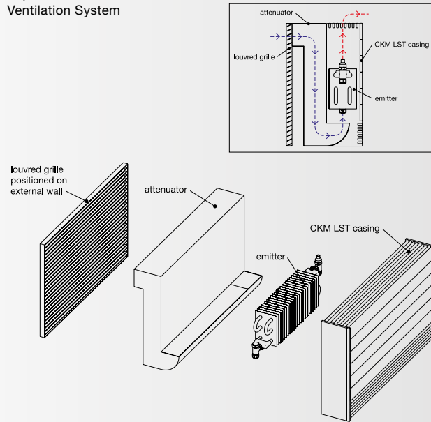
Exploded view of Natural Ventilation System
