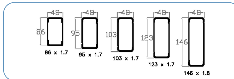
Boxed Beam Type
