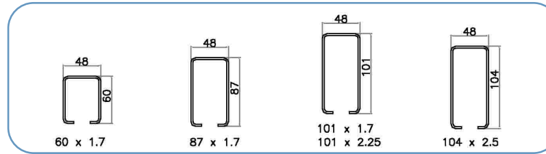
Open Beam Type
