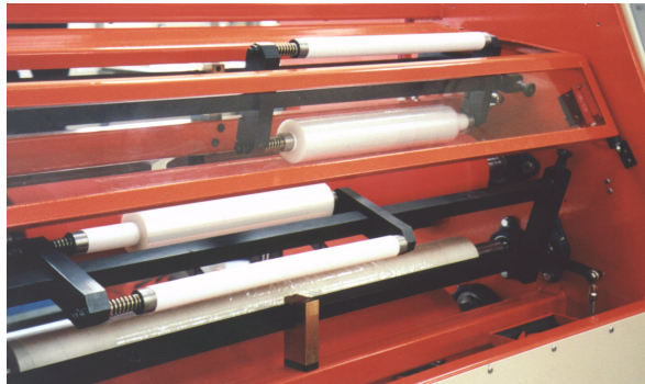
Twin turret arms for fast changeover.
