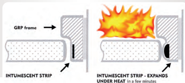
Dortek patented concealed intumescent strip
