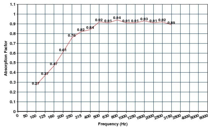
Internal Absorption Coefficient
