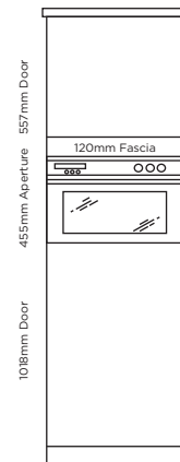
Compact Oven & Integrated Fridge Housing (B)
