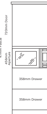
Microwave/ Compact Oven Housing (10G)
