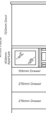
Microwave/ Compact Oven Housing (10D)
