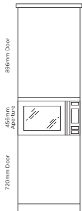
Microwave/ Compact Oven Housing (7A)
