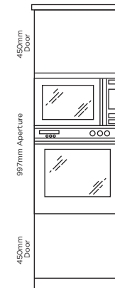
Single Oven & Microwave/ Compact Oven Housing (2A) †
