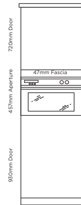
Compact Oven & Integrated Fridge Housing (D)
