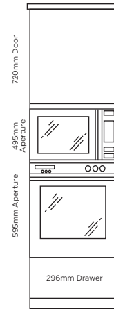
Single Oven & Microwave/ Compact Oven Housing (1A) †
