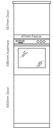
Single Oven & Integrated Fridge Housing (C)
