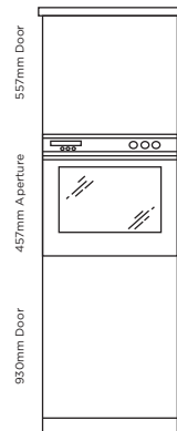
Compact Oven & Integrated Fridge Housing (B)
