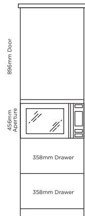
Microwave/ Compact Oven Housing (10G)
