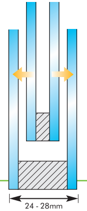
Document L* compliant, low E glass has a special coating that reflects heat back into your home
