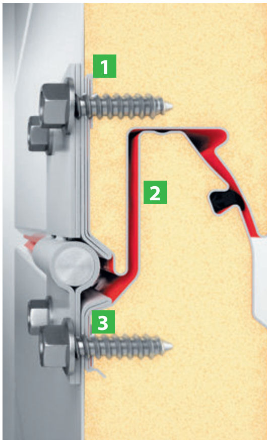
Closed contour of steel sheets
