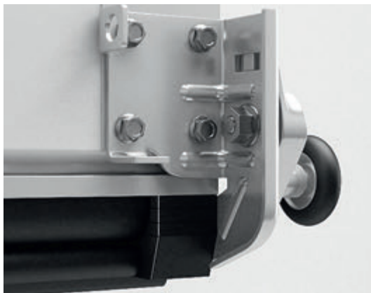
Bottom roller bracket of CLASSIC garage doors
