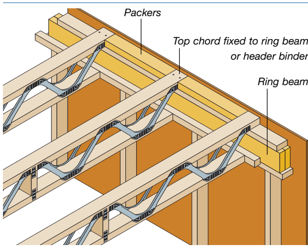
T15 • Proposed Arrangement for Timber Frame Construction
