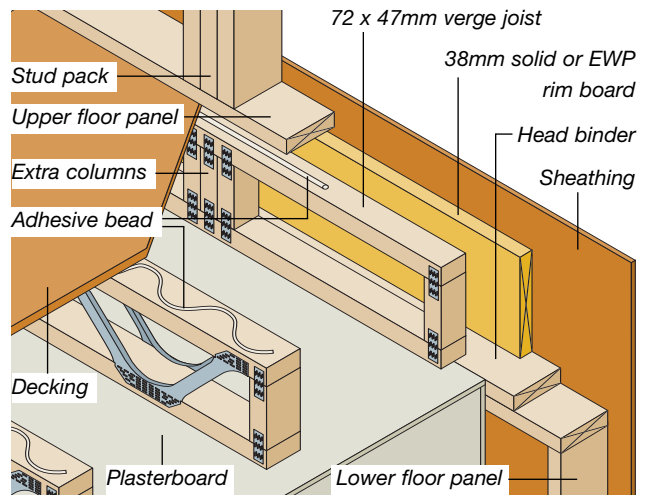
T14 • Proposed Arrangement for Timber Frame Construction
