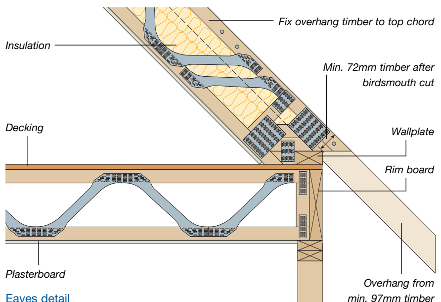
Eaves detail
