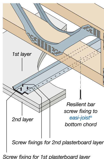
Resilient bar and plasterboard fixing
