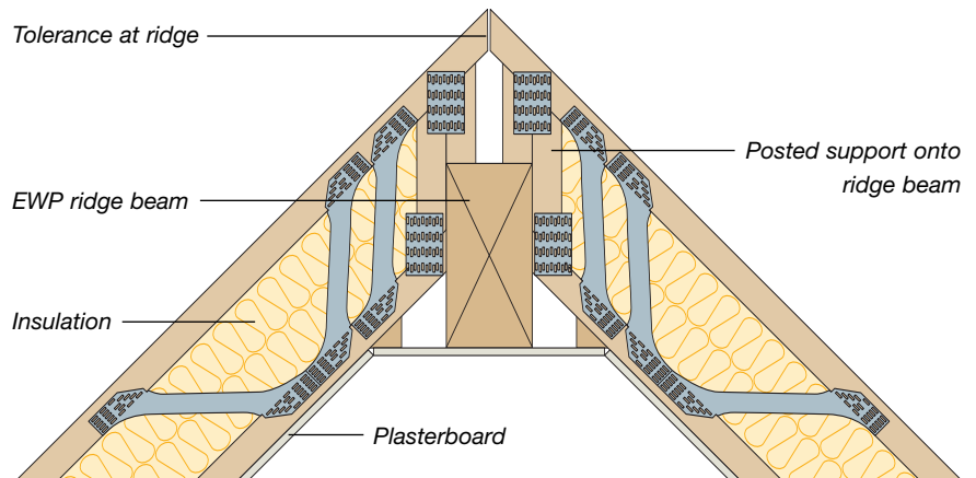
Ridge detail
