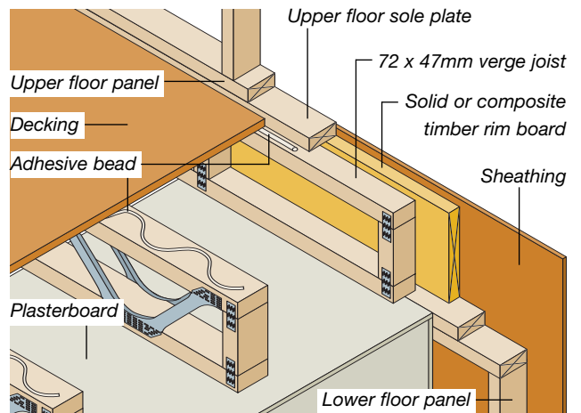
T16 • General Arrangement for Timber Frame Construction
