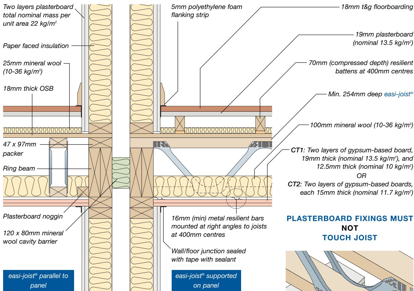
Separating floor construction (Robust Detail E-FT-3): 60 minutes fire resistance
