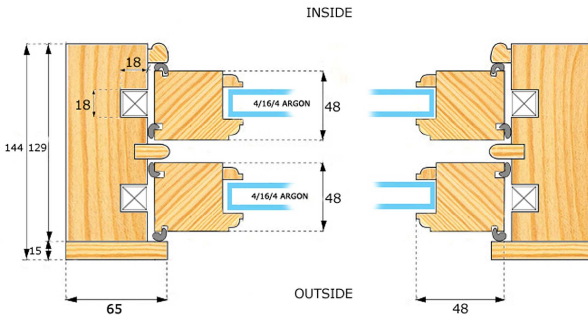
Sash window on spring balancer, view from the top
