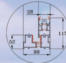
Section of bottom rail
