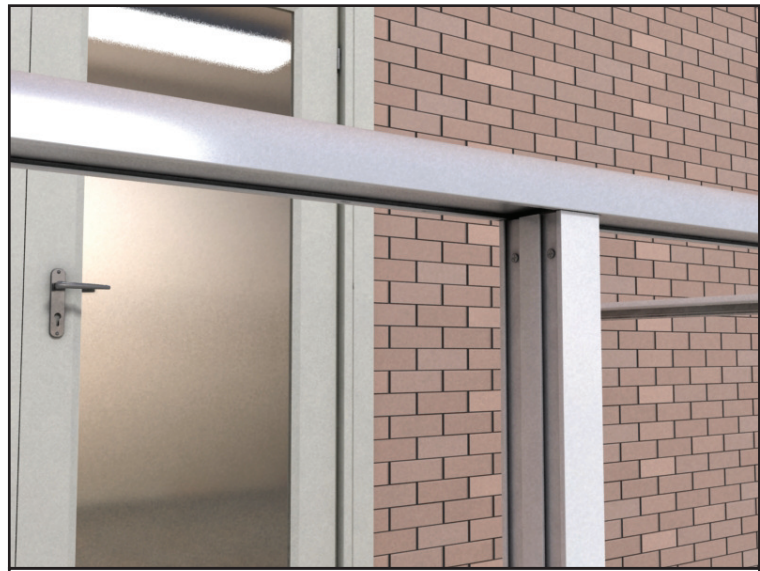
30 Fix the post into the post connector the No. 8 x1/2" S/tapping screws provided
