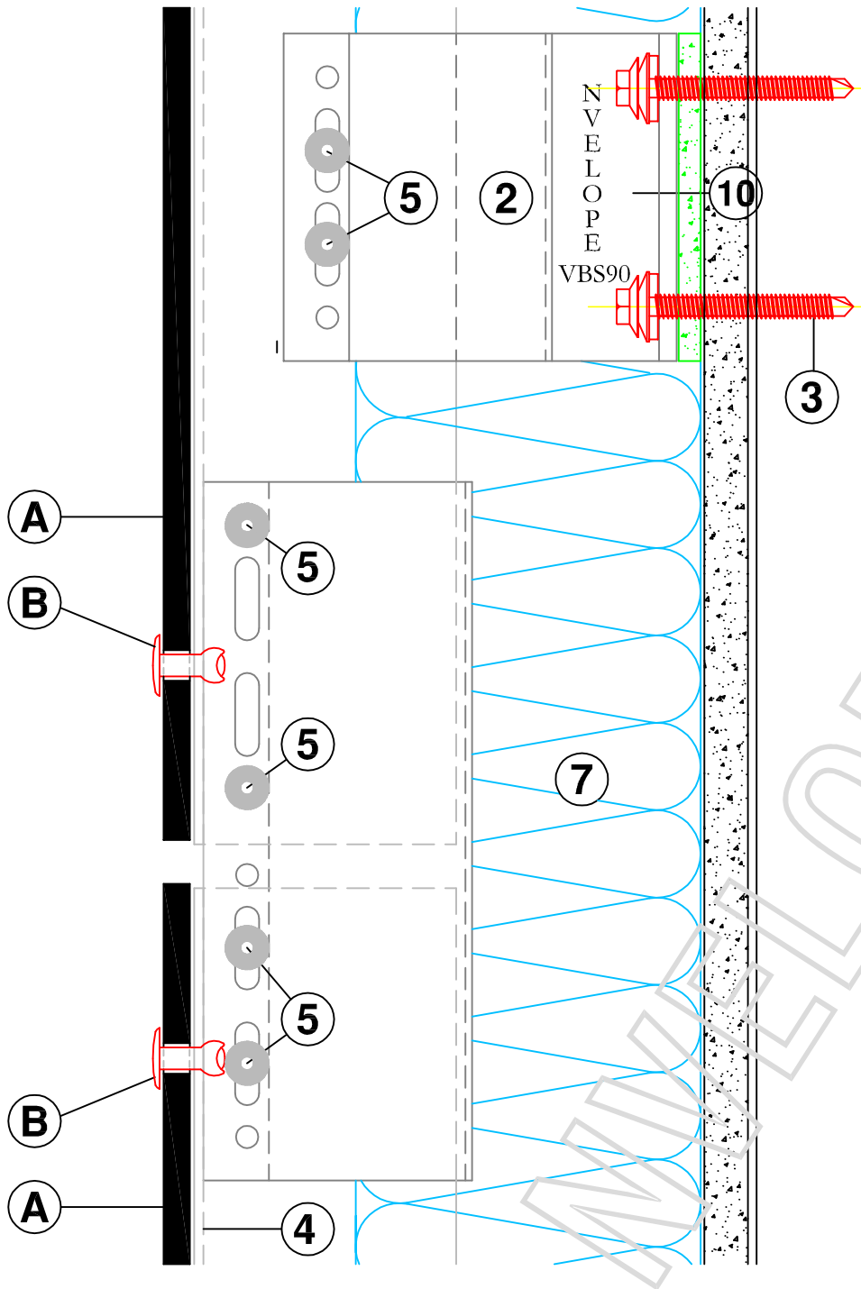
VERTICAL SECTION - RAIL JOINT OF PROFILE
