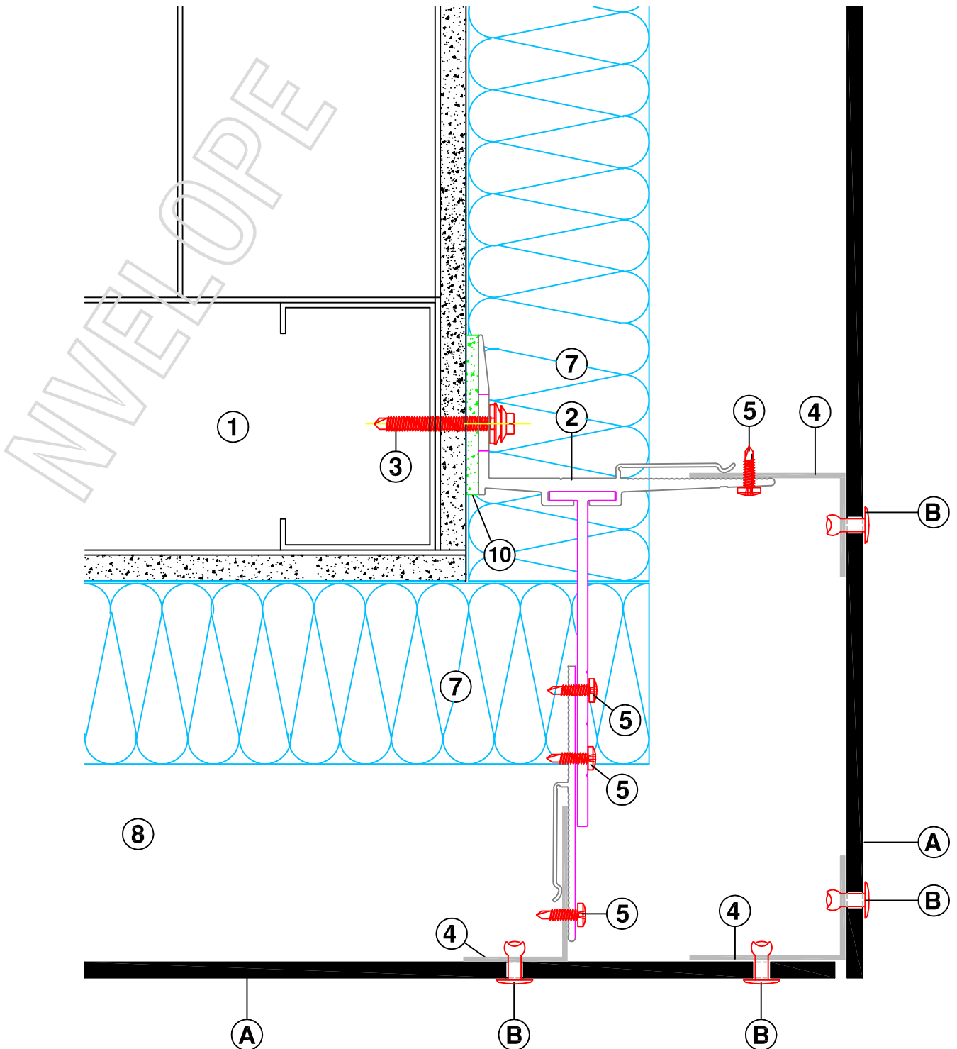
HORIZONTAL SECTION - EXTERNAL CORNER - WITH CORNER BRACKET
