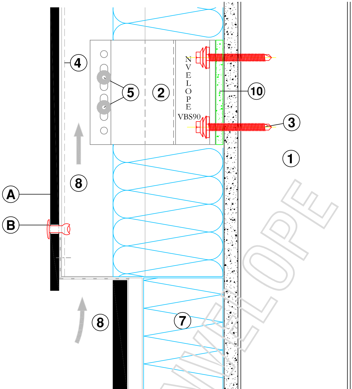
VERTICAL SECTION - BASE OF CLADDING
