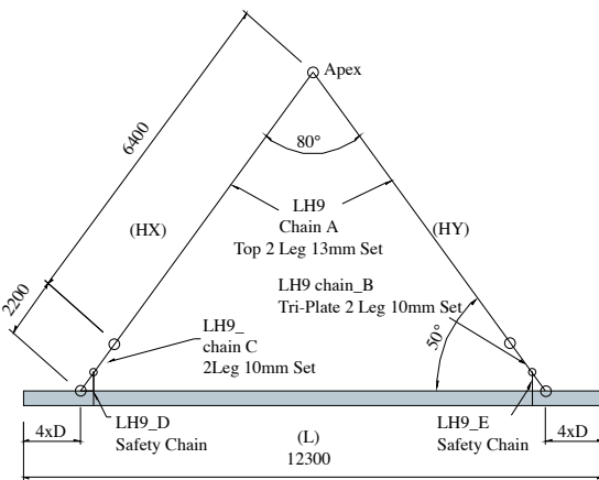
(LH9) Small Chain set for 9 Core Units 75 Plank to 260 Deep Units
