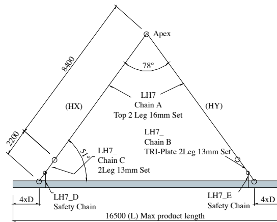
(LH7) Large Chain sling for 7 Core Units 300 to 450 Deep Units
