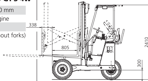
(Basic dimensions F3 253 GT-S 4W)
