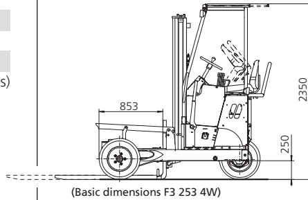
(Basic dimensions F3 253 4W)
