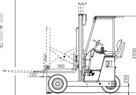
(Basic dimensions F3 253 4W)
