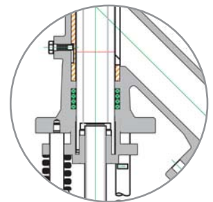
Detail: 26FR – Super Closure
