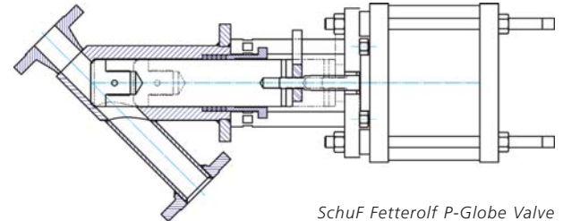
SchuF Fetterolf P-Globe Valve
