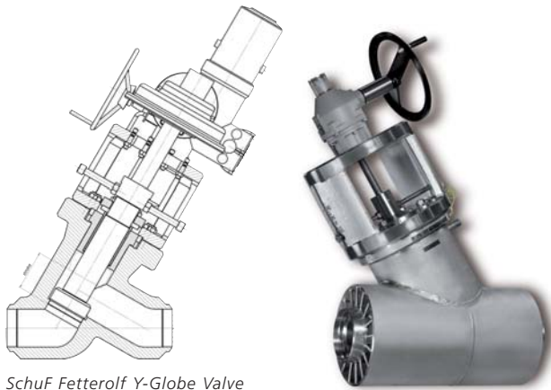
SchuF Fetterolf Y-Globe Valve
