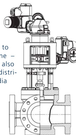
4-Way SwitchPlug Valve
