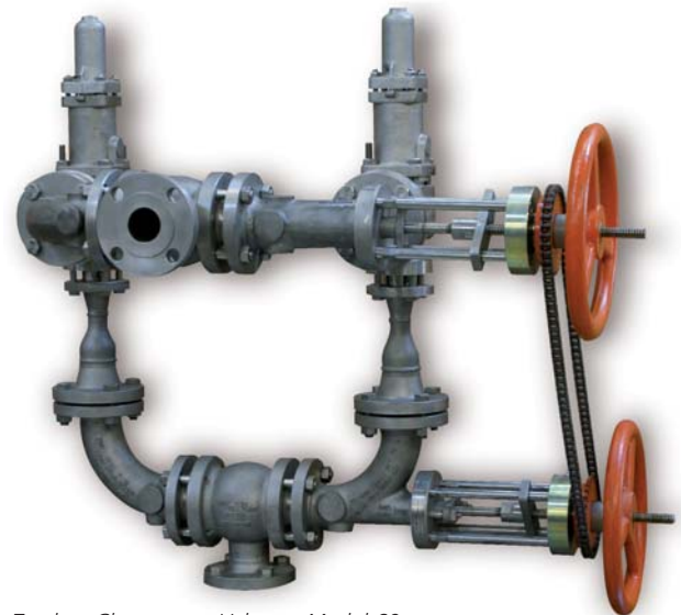
Tandem Changeover Valve – Model 69
