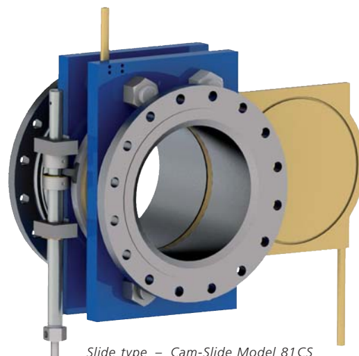
Slide type – Cam-Slide Model 81CS
