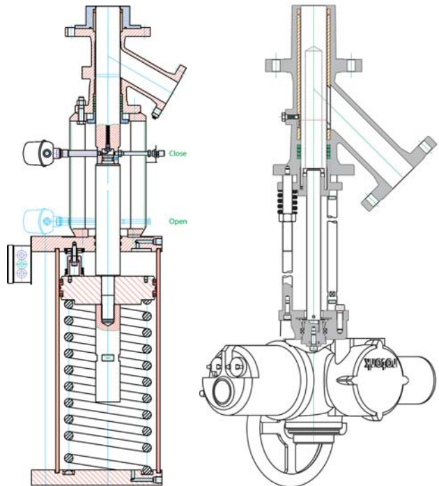
Ram drain valve – Model 28KR
