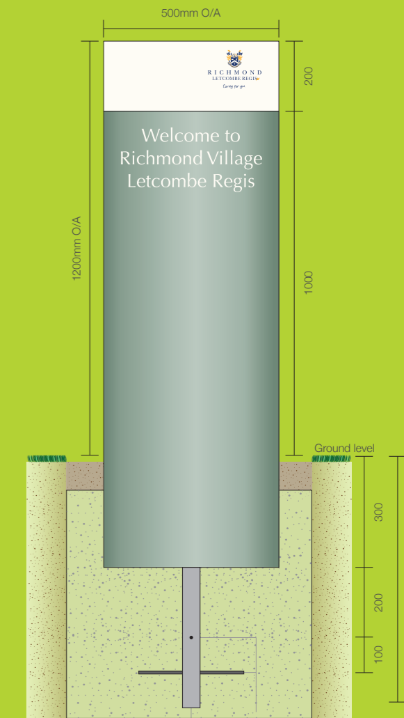
50mm x 50mm steel box section, fixed into void and mechanically fixed at top and bottom
