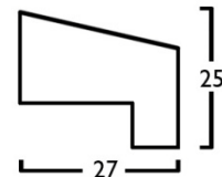
H/W Rebated Glazing Bead
