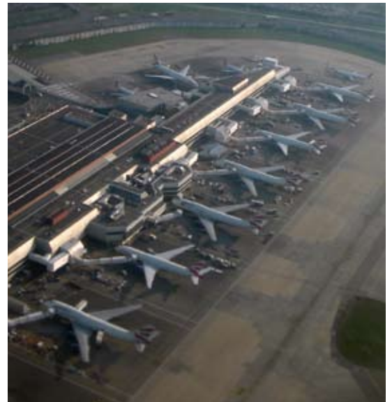
Rockbond Admix 201 and Admix 402 used to accelerated high strength microsilica concrete on the taxi ways and hard standing areas at Heathrow Airport.
