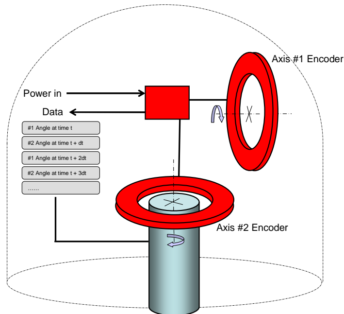
Figure 2 - Tandem Encoder schematic
