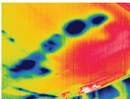
Also a lot of damage on the bottom of this inlet cowl can be seen on this thermal image.
