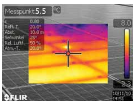
The Picture-in-Picture feature allows the user to overlay the thermal image directly over the corresponding visible image. At the push of a button the user can simply move, resize, and reshape thermal images inside the visual image.
