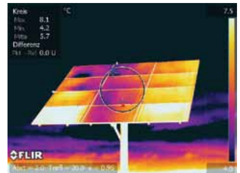
The hot spots on this thermal image taken from the front of the solar panel might seem to indicate that a multitude of cells are working inefficiently.
