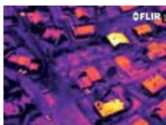
The buildings with yellow colored roofs show there is a moisture or insulation problem.
