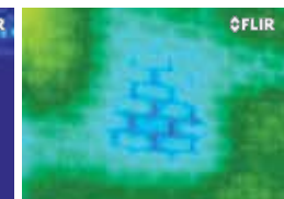
Missing insulation in parts of the wall.
