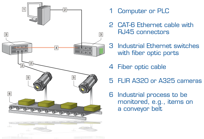
Figure 4. Typical Go/No-Go inspection system using IR cameras.
