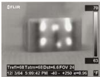
Figure 3. Machine vision box seal quality control
