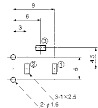
HOLE LAYOUT (BOTTOM VIEW)
