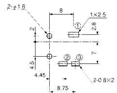
HOLE LAYOUT (BOTTOM VIEW)
