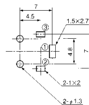
HOLE LAYOUT (BOTTOM VIEW)
