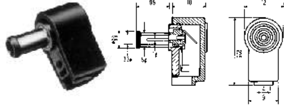
MP-204L RIGHT ANGLE
