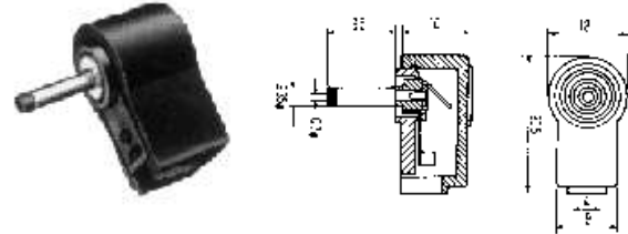
MP-201L RIGHT ANGLE
